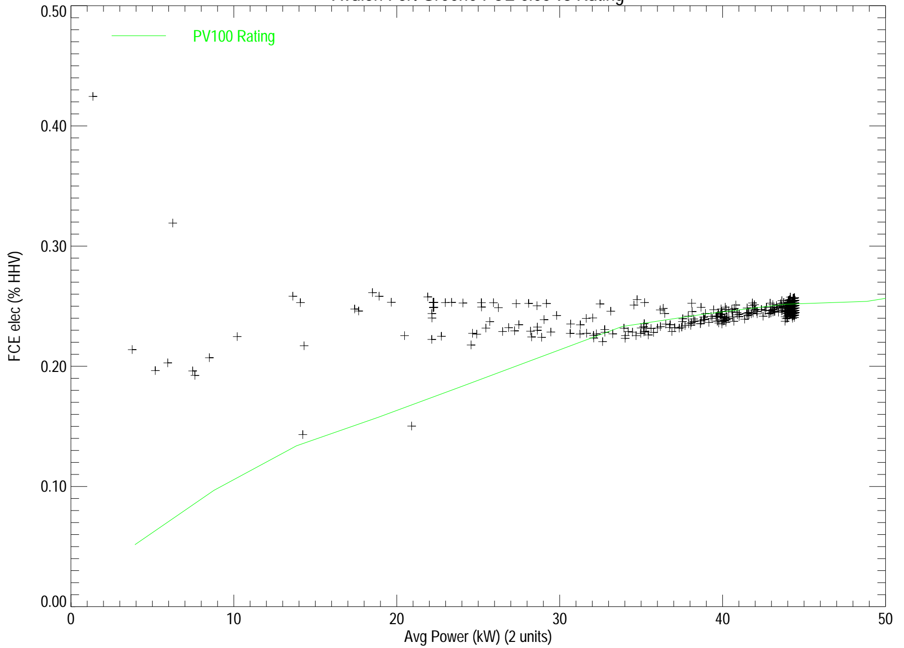
Avalon Fort Greene FCE elec vs Rating
