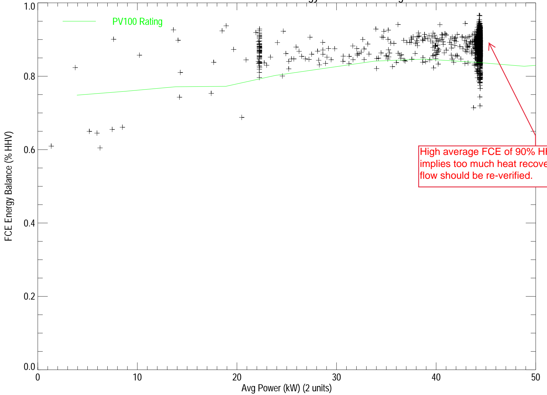
Avalon Fort Greene Total Energy Balance vs Rating
