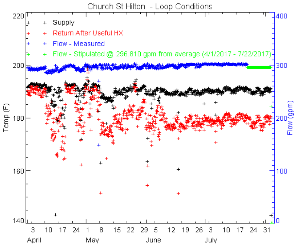
Figure 2. Loop Conditions with Measured and Stipulated Flow
