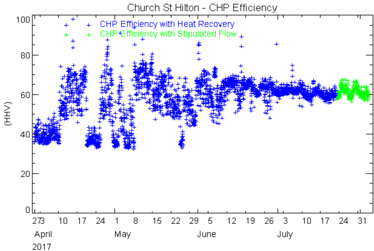
Figure 4. CHP Efficiency with Measured and Stipulated Flow
