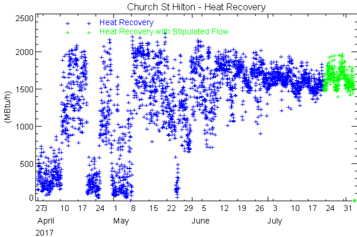
Figure 3. Heat Recovery with Measured and Stipulated Flow
